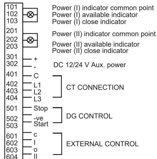
Connection Diagram Model L
