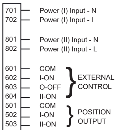
Connection Diagram Model G
