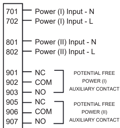
Connection Diagram Model X
