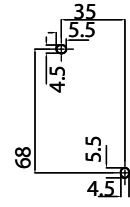
Screw mounting
